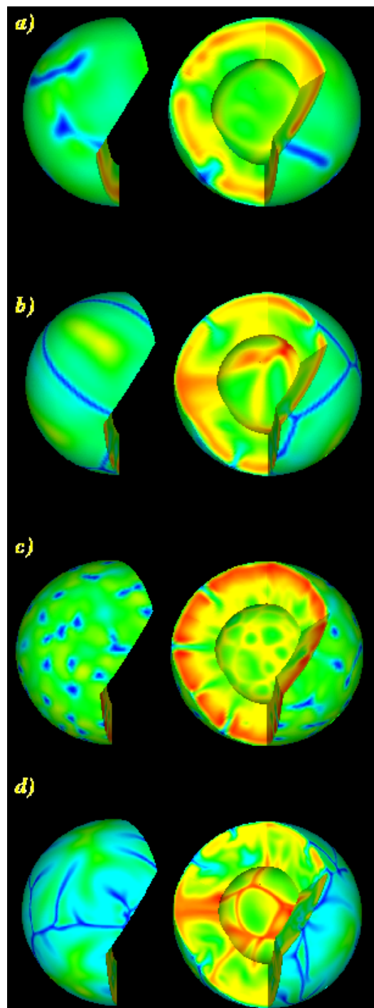
Plate 1. Purely internally heated convection in a spherical-shell model of the mantle with free-slip top and bottom surfaces, at moderate and high Ra , with and without a viscosity jump at 660km depth. Frame (a): Isoviscous mantle at Ra = 1.6 \times 10^5 . Frame (b): Same as (a), but with the viscosity of the upper mantle (above 660km) reduced by a factor of 30. Frame (c): Same as (a) except the entire mantle viscosity is reduced by 30 (thus Ra is larger by 30). Frame (d): Same as (b), except the viscosity of both layers is reduced by 10. Note that even while an increase in Ra causes more columnar downwellings (from frame (a) to frame (c)), a viscosity jump tends to re-inforce or restore the tendency for sheet-like downwellings (frame (d)). (After Bunge et al. [1996].)
