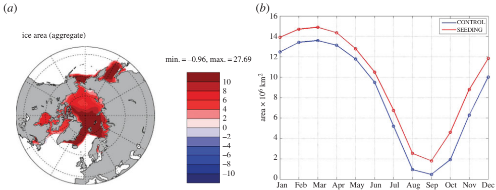
Figure 6. (a) Change in annual mean Arctic ice area (%) and (b) the annual cycle of NH sea ice area in simulations CONTROL and SEEDING ( 10^6 km 2 ).
