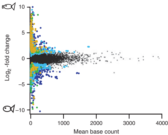
Fig. 4 Differential expression (mean base count to the \log_2 -fold change) by morph across all four lakes. Differentially expressed contigs between the two morphs (mean of the base counts from all the individuals of each morph to the \log_2 -fold change; FDR < 0.01) (Nicaragua = dark blue, Managua = light blue, Masaya = green, Apoyeque = yellow). Positive \log_2 -fold values indicate relative overexpression in thin-lipped morph; negative \log_2 -fold values indicate overexpression in thick-lipped morph.
