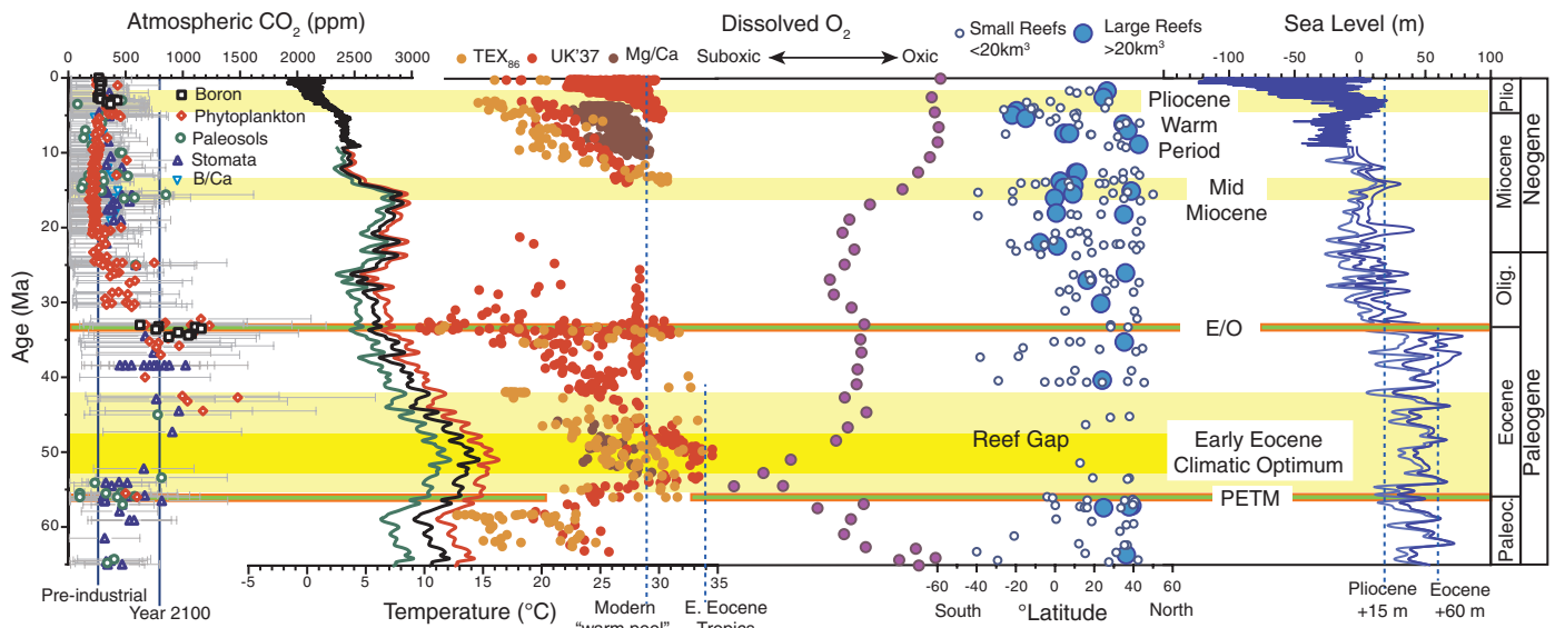
Fig. 2. Cenozoic record of major ecosystem drivers and responses. From left to right: Proxy evidence for atmospheric pCO_2 (14); vertical lines show the preindustrial pCO_2 (280 ppm) and estimated pCO_2 for year 2100 under a business-as-usual emissions scenario. Deep ocean temperature (15) estimated from oxygen isotope and Mg/Ca proxy evidence. Black line is long-term average for benthic foraminifera, red line is temperature adjusted for pH, and green line is temperature adjusted for seawater \delta^{18}O effects. Compilation of surface ocean temperature estimates from multiple organic matter and Mg/Ca proxies (as indicated by different colors) (37, 90–98); data are plotted with their published
