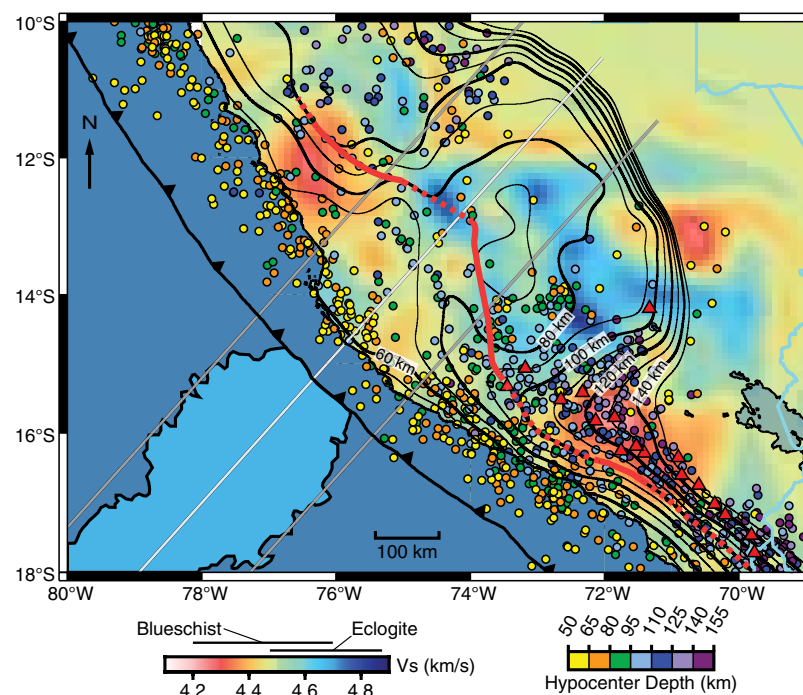
Figure 6. Comparison of subducted oceanic Moho slab contours and replotted surface-wave tomography at 75 km depth from Antonijevic et al. (2015) model. Earthquakes from International Seismological Centre (2011) catalogue ( \geq 4.5 magnitude, 50–150 km depth, from 1970 to 2013). Red line marks location of rapid decrease in slab Moho Ps arrival amplitude, indicating decrease in slab crust-mantle velocity contrast; line also corresponds to inboard edge of Dougherty and Clayton's (2015) dehydration-related slab top low-velocity layer. This boundary also corresponds to the transition from S-wave velocities characteristic of blueschist-facies materials (velocity range from Cao and Jung, 2016) to eclogite-facies materials (Worthington et al., 2013). See text for discussion.
