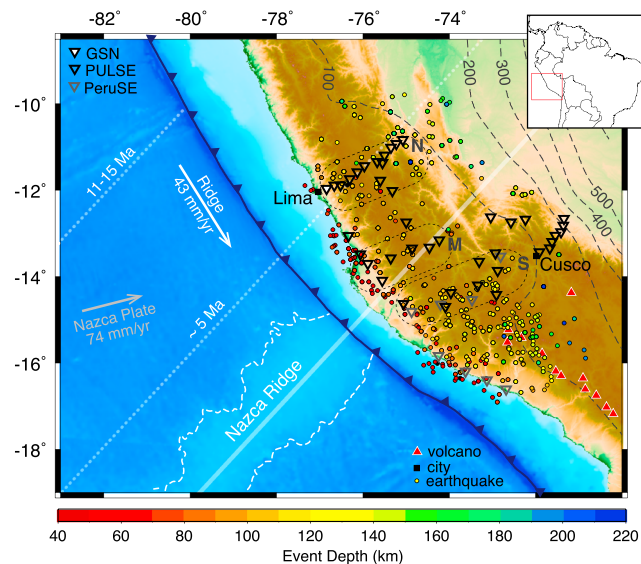
Figure 1. Tectonic setting and station locations. Slab contours (dashed dark grey lines) are from the Slab 1.0 model (unit: km) [Hayes et al., 2012]. Map shows distribution of seismicity (small circles colored by depth) and stations (triangles color coded by seismic network) used in this study. The northern, middle, and southern PULSE lines are enclosed by the thin dashed circles and labeled with N, M, and S, respectively. Thick white line shows continuation of the subducted Nazca Ridge. Dotted white lines show estimated position of the ridge in the past [Hampel, 2002]. Grey arrow represents the absolute plate motion of the Nazca plate from HS3-NUVEL1A [Gripp and Gordon, 2002]. Volcano locations (red triangles) are from Siebert and Simkin [2002].
