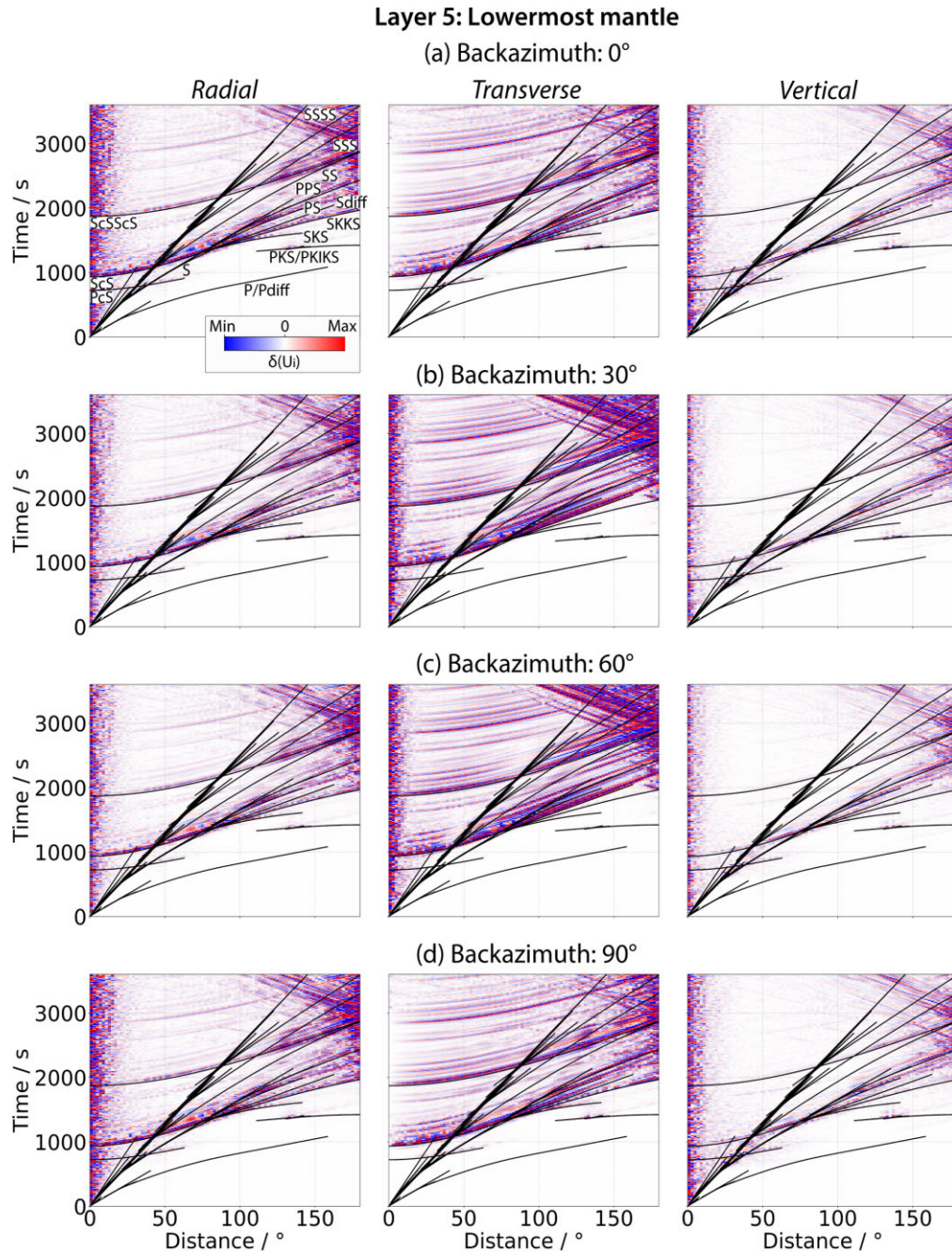
Figure 5. Differential displacement wavefield (color bar) as a function of distance for azimuths 0^\circ (first row), 30^\circ (second row), 60^\circ (third row) and 90^\circ (fourth row), calculated using a strike-slip source and elastic tensor arrangement 1 (Fig. 2c) for lowermost mantle anisotropy. Plotting conventions are as in Fig. 4.
