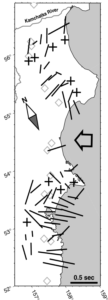
Figure 7. Averaged shear wave splitting measurements projected to mid-points along their respective rays. All observations that project to the depth between 50 and 100 km are averaged in spatial bins 0.5^\circ wide, with 50 per cent overlap between bins. Bins with four or more observations are plotted. Bars representing splitting measurements are aligned with the fast direction, scaled with delay, and registered to the centre of the bin. Crosses denote bins where averaged delay fell below 0.1 s. An open arrow shows subduction direction of the Pacific Plate. A compass sign (shaded to the south) is included for reference.
